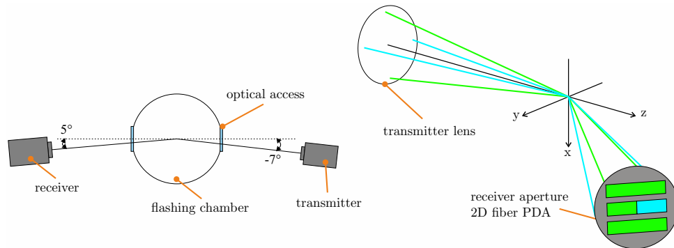
Figure 5. Optical set-up of 2D Fibre PDA system at test bench M3.3 (left) and receiver aperture of the used 2D fibre configuration (right)
