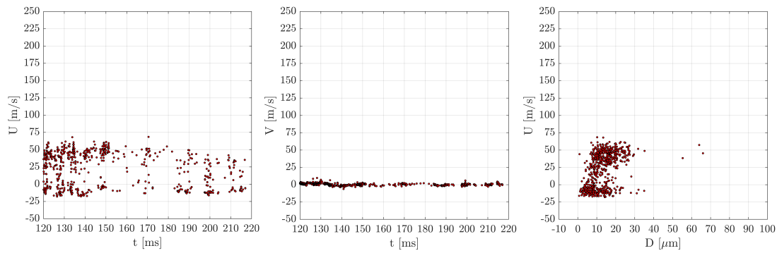
Figure 8. Vertical and horizontal velocities U (left) and V (middle) as functions of arrival time and vertical velocity U as function of the droplet diameter D (right) at position x/D = 0 and y/D = 30 in fully flashing LN2 sprays at T_{inj} = 89.7 K and p_{inj} = 4.4 \times 10^5 Pa
