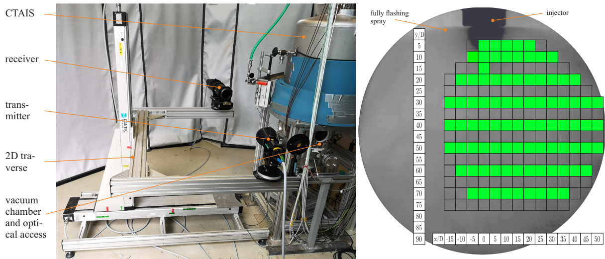
Figure 4. 2D Fibre PDA system at test bench M3.3 (left) and measurement positions in a fully flashing LN2 spray (right)
