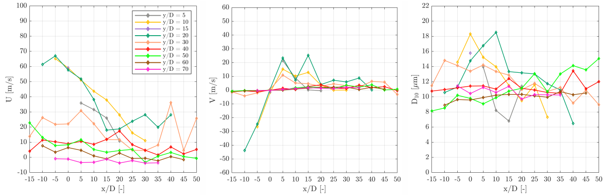
Figure 6. Arithmetical mean vertical velocity U (left), horizontal velocity V (middle) and mean diameter D_{10} (right) distributions in fully flashing LN2 sprays at T_{inj} = 89.7\text{ K} and p_{inj} = 4.4 \times 10^5\text{ Pa}
